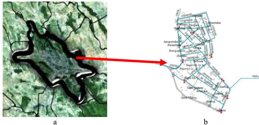
Fig. 4. Localization of the study area: a - the city of Iași; b - Aviation Plate area.
